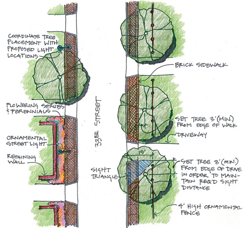
Typical Street Plan
