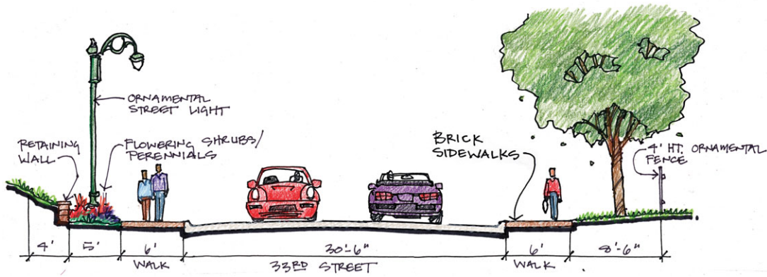
Typical 33rd Street Section
